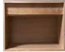
UNIT WITHOUT DOOR to be ordered with 1 large door W21 1/4" x D20 1/2" x H17 5/16" Ref. 5000
